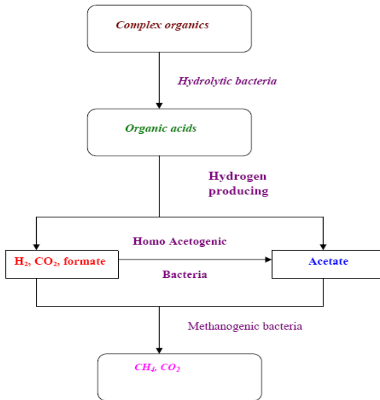
Figure 3: Biogas production process (Omer, 2003).
