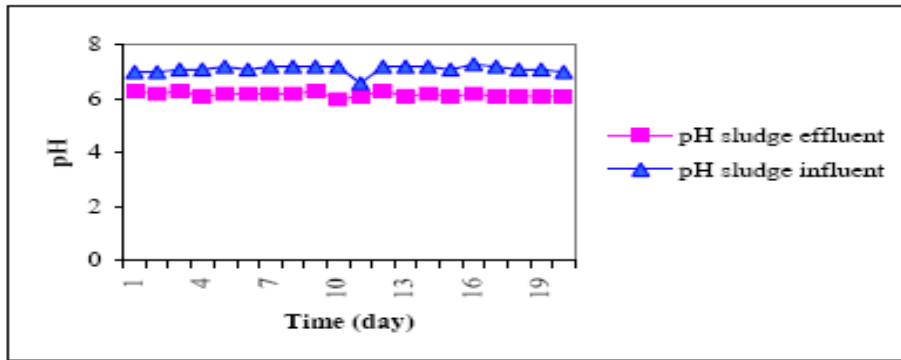
Figure 6: pH sludge before and after treatment in the digester (Omer, 2006).
