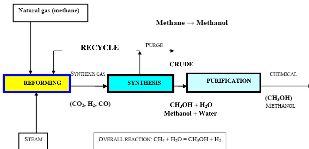
Figure 2: Schematic diagram shows methanol production (Omer, 2006).
