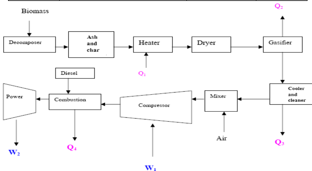
Figure 7: Advanced biomass power with diesel engine (Omer, 2006).
