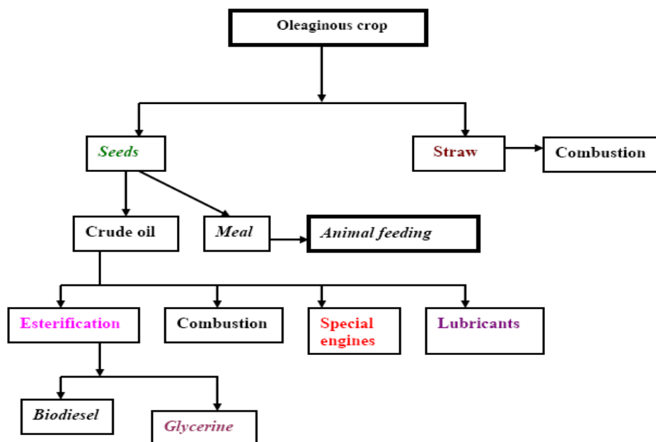
Figure 9: Flow chart of biodiesel production (Omer, 2006).
